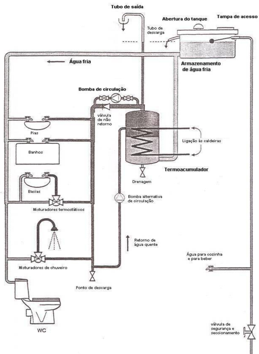
Figura 11: Sistema gravítico com recirculação (retirado de “ Legionnaires’ s disease – The control of legionella bactéria in water systems” – HSC (Health Safety Commission “
